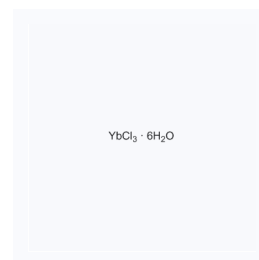
1182213 CAS: 10035-01-5
