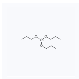
1157725 CAS: 6742-69-4
