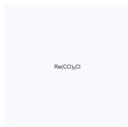
1182431 CAS: 14099-01-5
