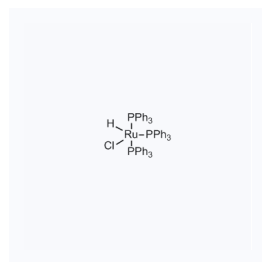
1152720 CAS: 55102-19-7
