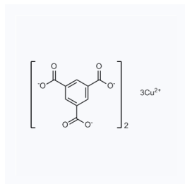
1181624 CAS: 51937-85-0
