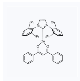
1155949 CAS: 920739-11-3
