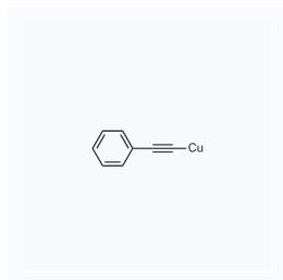
1181673 现货 CAS: 13146-23-1
