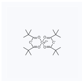
1105824 现货 CAS: 14040-05-2
