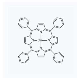
1156668 CAS: 14172-91-9
