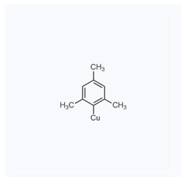
1181683 现货 CAS: 75732-01-3
