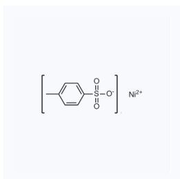
1156021 CAS: 6944-05-4
