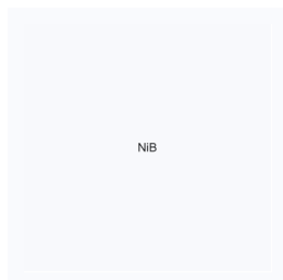
1181515 现货 CAS: 12007-00-0
