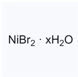
1181519 现货 CAS: 207569-11-7
