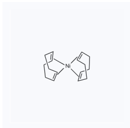
1105832 现货 CAS: 1295-35-8
