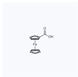
1019126 现货 CAS: 1271-42-7
