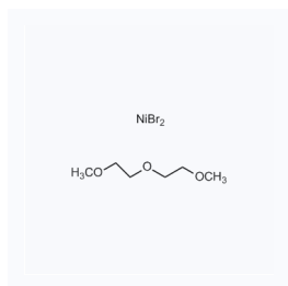
1169659 CAS: 312696-09-6
