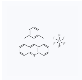
1176206 现货 CAS: 872205-11-3
