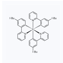
1181194 CAS: 474948-23-7
