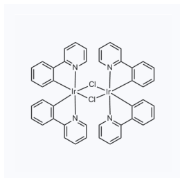
1046774 现货 CAS: 92220-65-0
