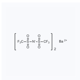
1177067 CAS: 168106-22-7
