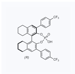
1164012 现货 CAS: 791616-70-1
