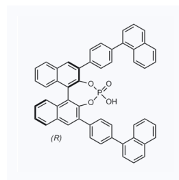
1163864 CAS: 1450925-06-0
