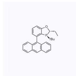
1161752 现货 CAS: 1884594-03-9
