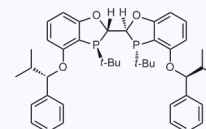
1184276 CAS: 2169292-11-7
