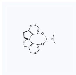
1107649 现货 CAS: 443965-14-8
