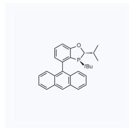
1161713 现货 CAS: 1891002-61-1
