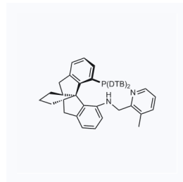
1161575 现货 CAS: 2241655-67-2
