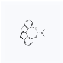
1133042 现货 CAS: 443965-10-4
