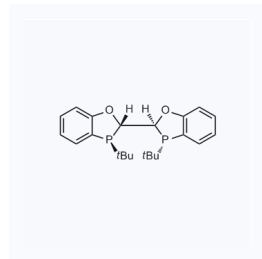
1159009 现货 CAS: 1202033-17-7
