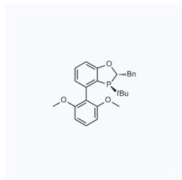
1161732 现货 CAS: 1373432-13-3
