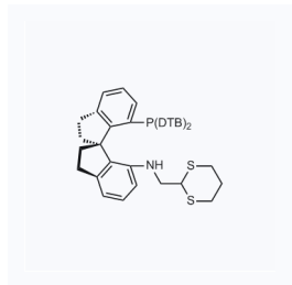
1205297 现货 CAS: 2177266-21-4
