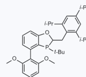
1184256 CAS: 1908442-13-6
