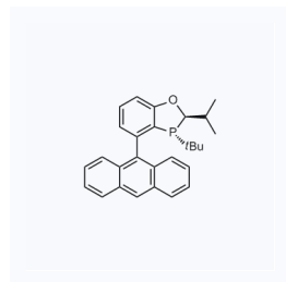
1161711 现货 CAS: 1891002-60-0
