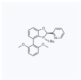
1184263 现货 CAS: 1542796-11-1
