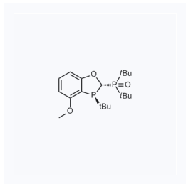
1161696 现货 CAS: 1788085-46-0
