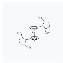
1176015 CAS: 540475-73-8
