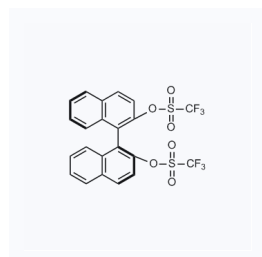
1019250 现货 CAS: 128544-05-8
