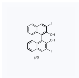
1157850 现货 CAS: 287111-93-7
