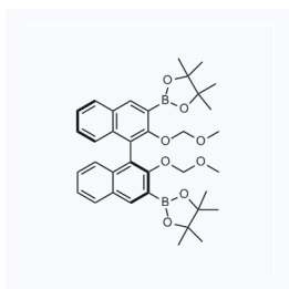
1157601 CAS: 260441-99-4
