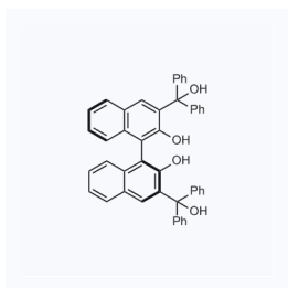
1157605 CAS: 309269-73-6
