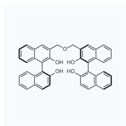
1158215 CAS: 336800-79-4
