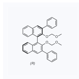
1158225 CAS: 428874-67-3
