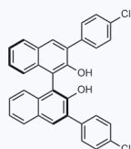
1158195 CAS: 1204609-08-4
