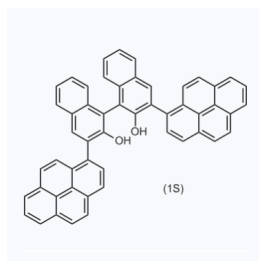
1161781 CAS: 1854074-57-9
