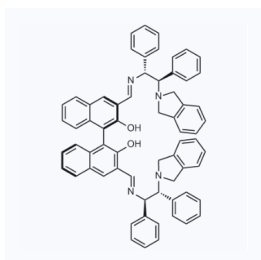
1155767 CAS: 1620285-48-4
