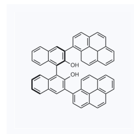
1212247 CAS: 1854074-51-3
