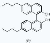
1167246 CAS: 208715-27-9
