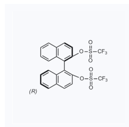
1019063 现货 CAS: 126613-06-7
