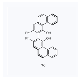
1157073 现货 CAS: 147702-16-7
