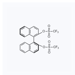
1019250 现货 CAS: 128544-05-8
