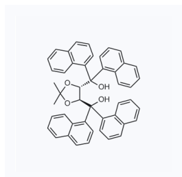
1157002 CAS: 171086-52-5
