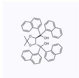
1105843 现货 CAS: 137536-94-8
