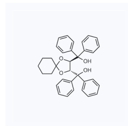
1157560 CAS: 114026-76-5
