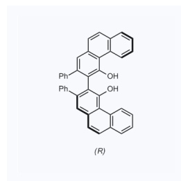
1157073 现货 CAS: 147702-16-7
