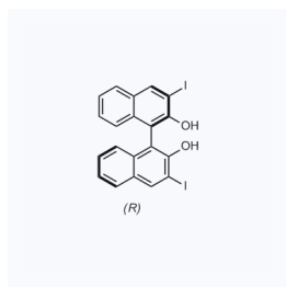
1157850 现货 CAS: 287111-93-7
