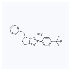
1155785 CAS: 862095-77-0
