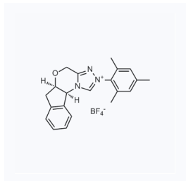
1157791 现货 CAS: 925706-31-6
