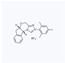
1157769 现货 CAS: 1061311-82-7
