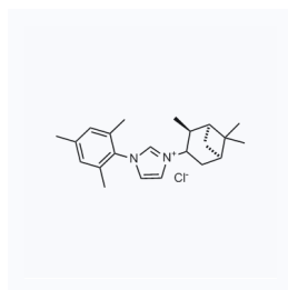
1176874 CAS: 1583244-12-5
