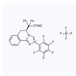
1174040 CAS: 1710476-23-5
