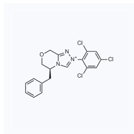
1174048 CAS: 1612251-12-3
