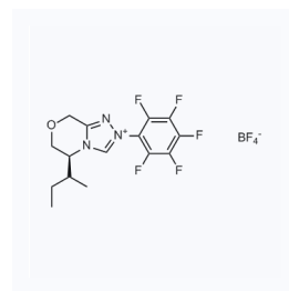
1158572 CAS: 1449522-21-7
