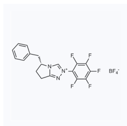
1163525 CAS: 1072808-07-1
