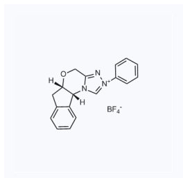
1157783 现货 CAS: 463326-74-1
