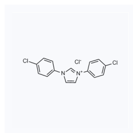
1105844 现货 CAS: 141556-46-9
