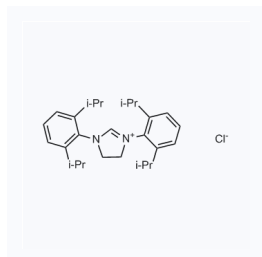
1027567 现货 CAS: 258278-25-0
