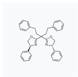
1168517 CAS: 583058-02-0
