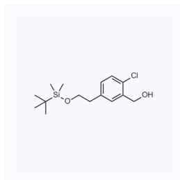
1173647 现货 CAS: 1911653-46-7
