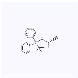
1105949 现货 CAS: 603045-12-1
