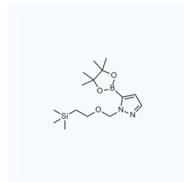
1162452 CAS: 903550-12-9
