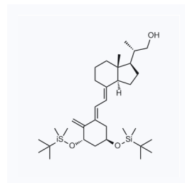
1057481 现货 CAS: 128387-35-9
