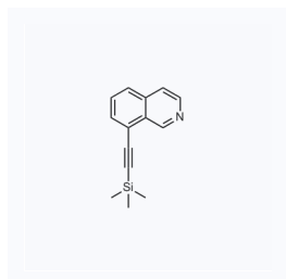
1048543 现货 CAS: 1823440-48-7
