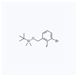
1164837 CAS: 1400757-50-7
