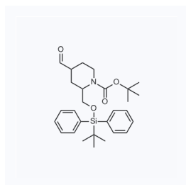
1119076 CAS: 1630906-46-5
