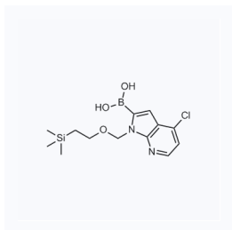
1123844 CAS: 888721-03-7
