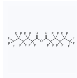
1192215 CAS: 308-13-4
