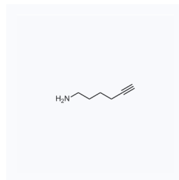
1177234 CAS: 15252-45-6
