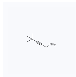
1201057 CAS: 113439-90-0
