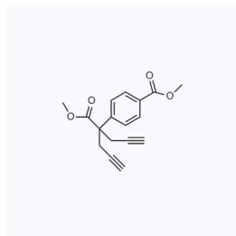
1060046 现货 CAS: 1026380-17-5
