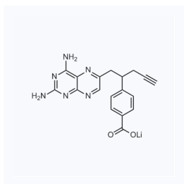
1060045 现货 CAS: 1445586-53-7
