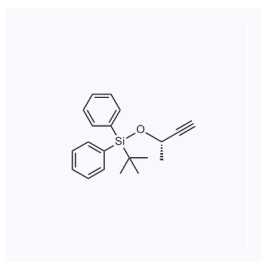
1105949 现货 CAS: 603045-12-1
