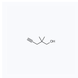
1183439 CAS: 107540-03-4
