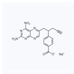
1066972 现货 CAS: 1445586-50-4
