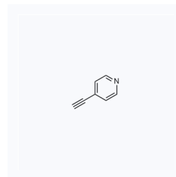
1062106 CAS: 2510-22-7
