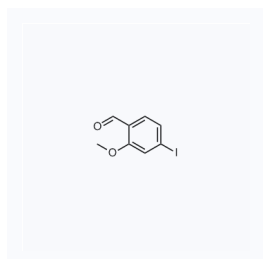
1202011 现货 CAS: 139102-37-7
