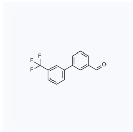
1115980 现货 CAS: 126091-24-5
