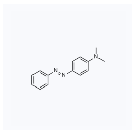
1135512 现货 CAS: 60-11-7
