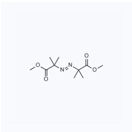
1201080 CAS: 2589-57-3
