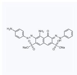
1057000 现货 CAS: 288323-10-4
