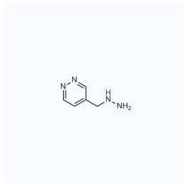
1125796 CAS: 1363380-98-6
