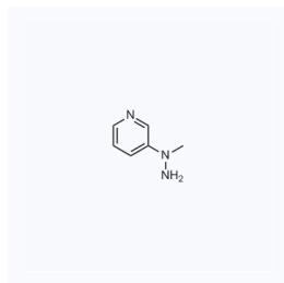
1159802 CAS: 99979-60-9
