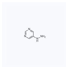
1127922 CAS: 1262021-60-2
