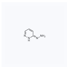
1065163 CAS: 40972-16-5
