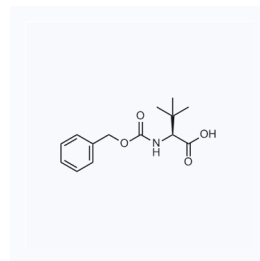
1038401 现货 CAS: 62965-10-0
