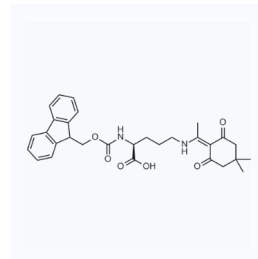
1027941 现货 CAS: 269062-80-8
