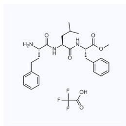
1066778 现货 CAS: 868539-99-5
