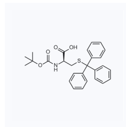
1045440 现货 CAS: 87494-13-1
