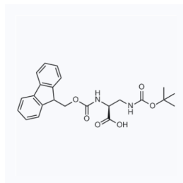
1022952 现货 CAS: 162558-25-0
