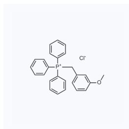
1111580 CAS: 18880-05-2
