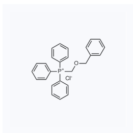
1108249 CAS: 75772-01-9
