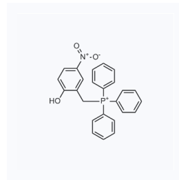
1170943 CAS: 741624-27-1
