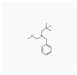
1046916 现货 CAS: 93102-05-7
