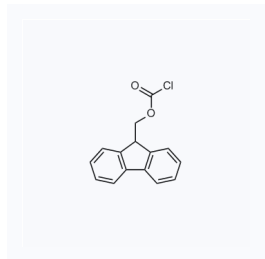
1028438 现货 CAS: 28920-43-6
