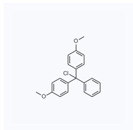
1032118 现货 CAS: 40615-36-9
