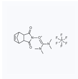
1025611 CAS: 208462-94-6
