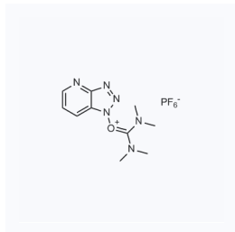
1021961 现货 CAS: 148893-10-1
