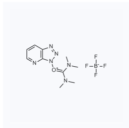
1045371 现货 CAS: 873798-09-5
