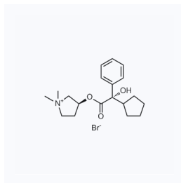
1191429 CAS: 201667-20-1
