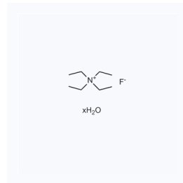
1047645 现货 CAS: 98330-04-2
