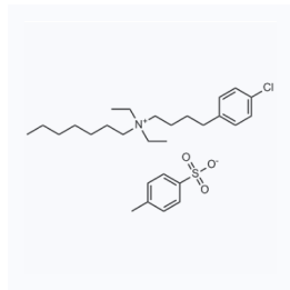
1061673 现货 CAS: 92953-10-1
