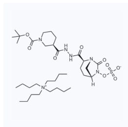
1164687 CAS: 1436862-01-9
