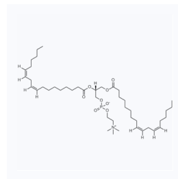
1047851 CAS: 998-06-1
