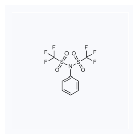
1031201 现货 CAS: 37595-74-7
