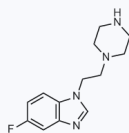
1143952 CAS: 2097937-55-6
