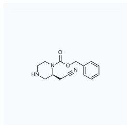
1166383 现货 CAS: 2158302-01-1
