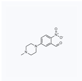
1161117 现货 CAS: 904895-82-5
