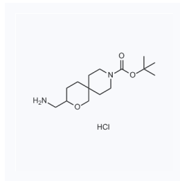
1110640 CAS: 2177257-50-8
