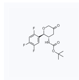
1047972 CAS: 951127-24-5
