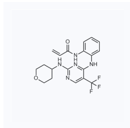
1125198 CAS: 1788058-89-8
