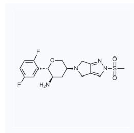
1127021 CAS: 1443380-88-8
