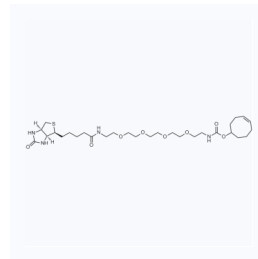
1185150 CAS: 2183440-30-2
