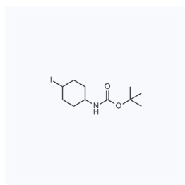
1111647 现货 CAS: 1179986-79-8
