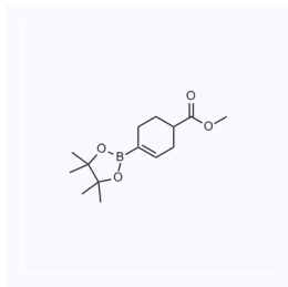
1064439 现货 CAS: 151075-20-6
