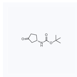
1118674 现货 CAS: 167298-40-0
