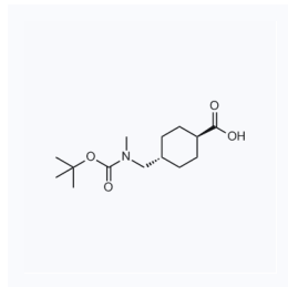
1198547 现货 CAS: 165947-29-5
