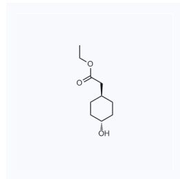
1061878 现货 CAS: 116941-05-0
