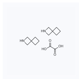
1122672 现货 CAS: 1365639-13-9
