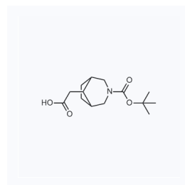
1107708 现货 CAS: 1250996-75-8
