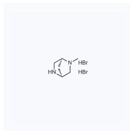
1124189 现货 CAS: 125224-62-6
