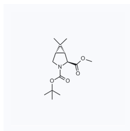
1070178 现货 CAS: 569679-06-7
