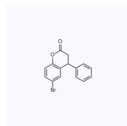
1058273 现货 CAS: 156755-23-6
