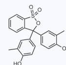
1079955 CAS: 1733-12-6
