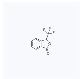
1051393 现货 CAS: 887144-94-7
