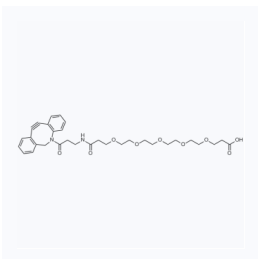
1162807 CAS: 1870899-46-9
