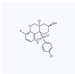
1058453 现货 CAS: 944949-06-8
