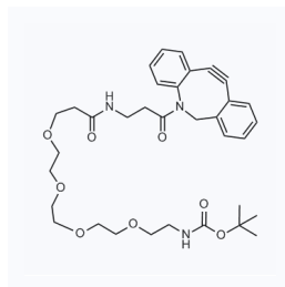
1178624 CAS: 1255942-12-1
