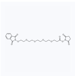
1175677 CAS: 1415328-95-8
