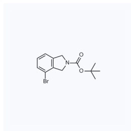
1062991 现货 CAS: 1035235-27-8
