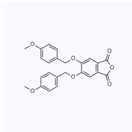
1198727 CAS: 1609071-04-6
