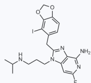
1050087 CAS: 1799421-10-5
