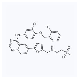
1171057 CAS: 1393112-45-2
