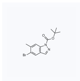
1171797 现货 CAS: 1305320-67-5
