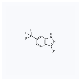
1104591 现货 CAS: 1000341-21-8
