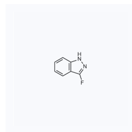
1124960 现货 CAS: 66607-26-9
