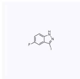
1069101 现货 CAS: 858629-06-8
