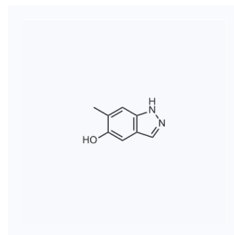
1049788 现货 CAS: 478832-60-9
