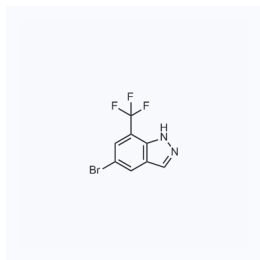
1111953 现货 CAS: 1374258-43-1
