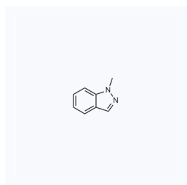
1125383 现货 CAS: 13436-48-1
