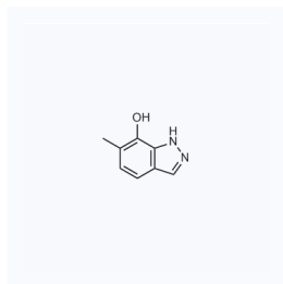
1127410 现货 CAS: 92224-25-4
