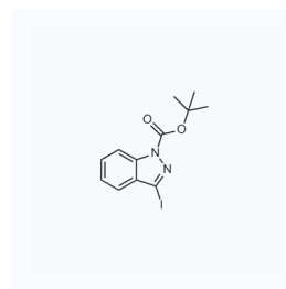
1064429 CAS: 290368-00-2
