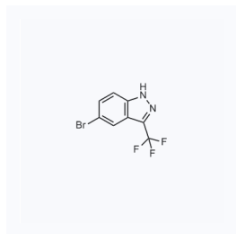
1088961 现货 CAS: 57631-11-5
