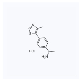
1066760 现货 CAS: 1948273-01-5
