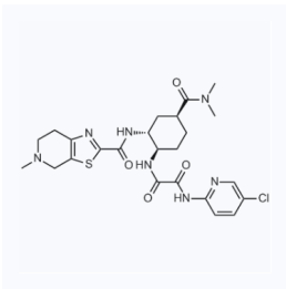
1124771 CAS: 500572-10-1
