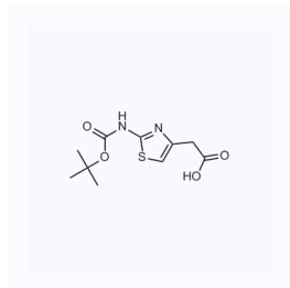
1051609 现货 CAS: 89336-46-9
