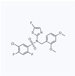
1105715 现货 CAS: 1788874-30-5
