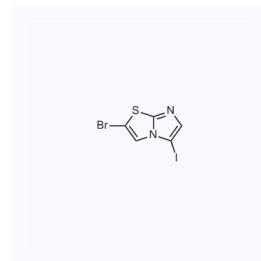
1057366 现货 CAS: 1379307-48-8
