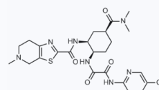
1124769 CAS: 1255529-25-9
