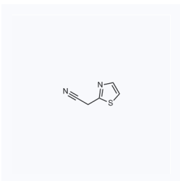
1122427 现货 CAS: 101010-74-6
