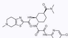
1124767 CAS: 1255529-27-1
