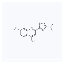
1058208 现货 CAS: 923289-21-8
