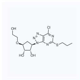
1080423 现货 CAS: 1354945-69-9
