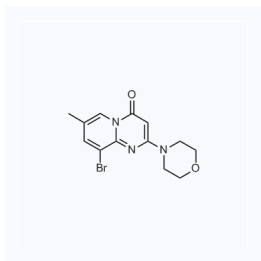
1058522 现货 CAS: 351002-16-9
