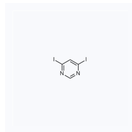
1169388 现货 CAS: 19646-06-1
