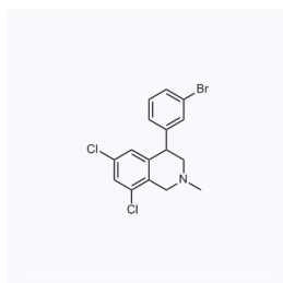
1066866 现货 CAS: 543737-10-6
