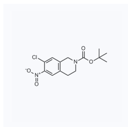
1154010 现货 CAS: 912846-74-3
