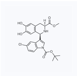
1066684 现货 CAS: 1395347-28-0
