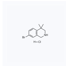
1205353 CAS: 1203684-66-5
