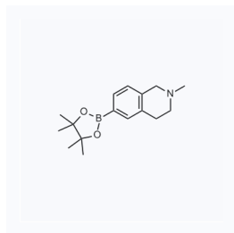
1202097 CAS: 922718-57-8
