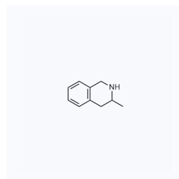
1068609 CAS: 29726-60-1
