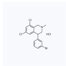
1121844 现货 CAS: 543739-81-7
