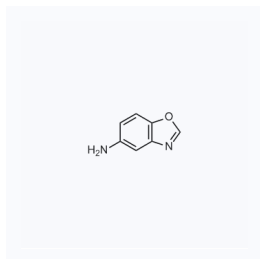
1108912 现货 CAS: 63837-12-7
