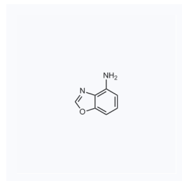
1200940 现货 CAS: 163808-09-1
