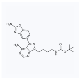
1172876 现货 CAS: 1887095-80-8
