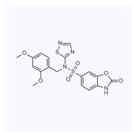
1105706 现货 CAS: 1432514-50-5
