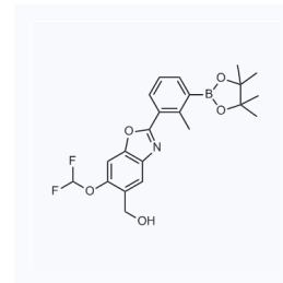
1198858
