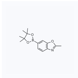
1107432 现货 CAS: 1408089-23-5
