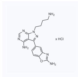
1168261 CAS: 1971086-51-7
