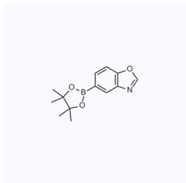
1062395 现货 CAS: 936902-12-4
