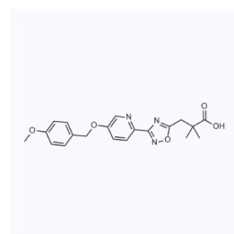
1060956 CAS: 917911-01-4
