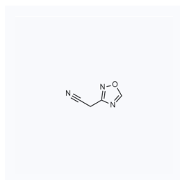
1155725 CAS: 809534-07-4
