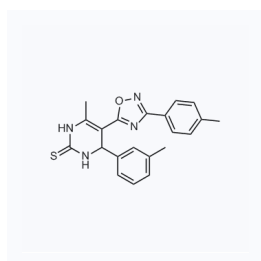
1141155 CAS: 892302-22-6
