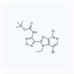
1057377 CAS: 842144-08-5
