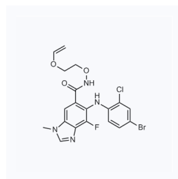
1058657 CAS: 606144-05-2
