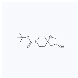
1053243 现货 CAS: 240401-09-6
