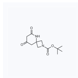
1048513 现货 CAS: 1105662-95-0
