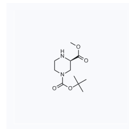
1058087 现货 CAS: 438631-77-7
