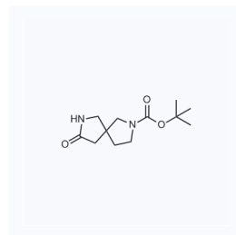
1108825 现货 CAS: 1251009-03-6
