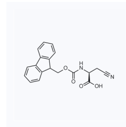
1172678 现货 CAS: 127273-06-7
