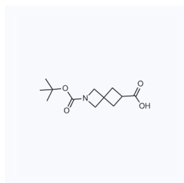
1049954 现货 CAS: 1211526-53-2
