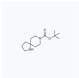
1065110 现货 CAS: 937729-06-1
