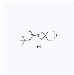
1057869 现货 CAS: 929302-18-1
